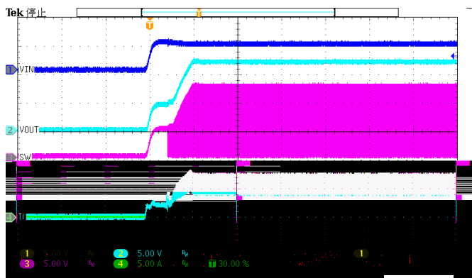
Figure 20. Power up(Iload=2A)
