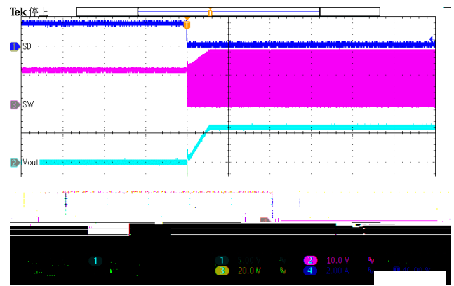
Figure 31. Shutdown remove
