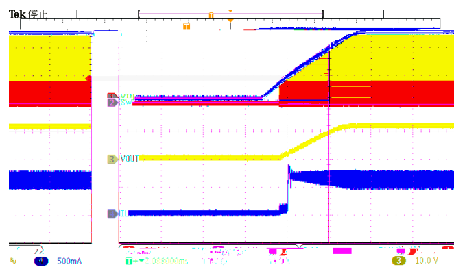
Figure 12. Power up
